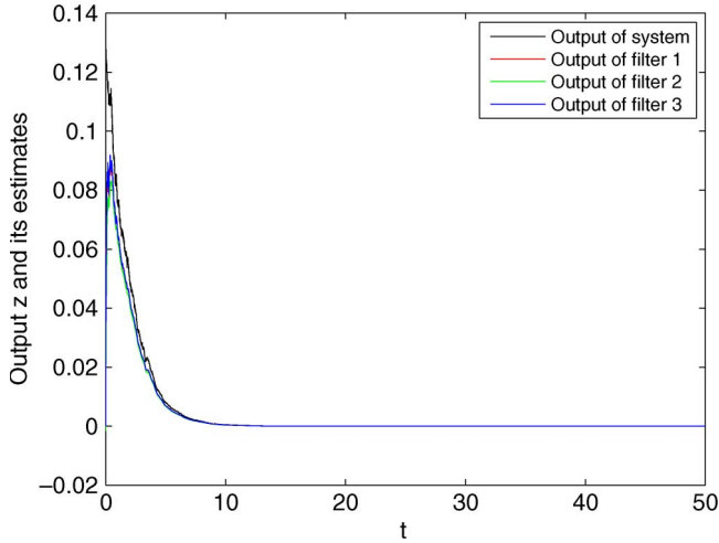
Fig. 1. Output z(t) and its estimates.
