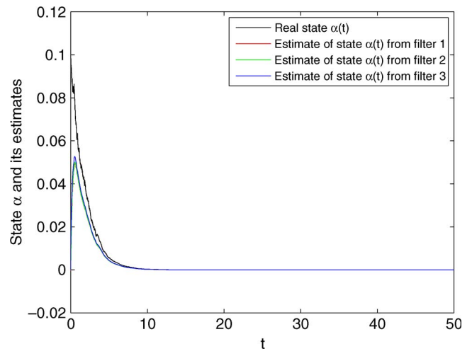
Fig. 4. State \alpha(t) and its estimates.
