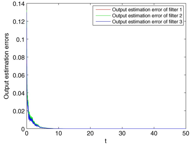
Fig. 2. Filtering errors \tilde{z}_i(t) , i = 1, 2, 3 .
