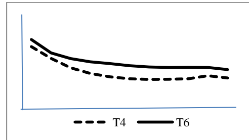
Figure 7: Pitch contour of T4 and T6 produced by the near-merger participant
