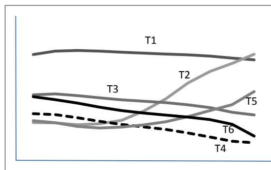
Figure 1: The pitch contours of the six contrastive tones in Hong Kong Cantonese
