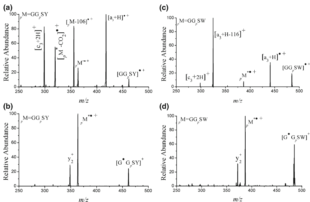
Figure 4. CID spectra of (a) [\text{GG}_p\text{SY}]^{\bullet+} , (b) [\text{G}_p\text{G}_p\text{SY}]^{\bullet+} , (c) [\text{GG}_p\text{SW}]^{\bullet+} , and (d) [\text{G}_p\text{G}_p\text{SW}]^{\bullet+}
