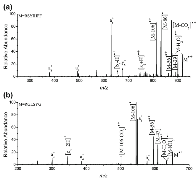
Figure 3. CID spectra of (a) [\text{RSYIHPF}]^{\bullet+} and (b) [\text{RGLSYG}]^{\bullet+}
