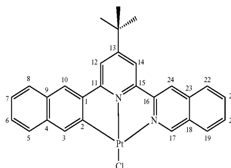
Complex 2
