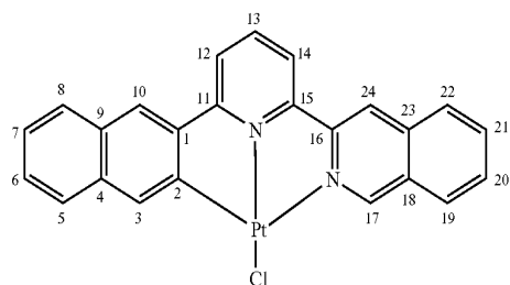
Complex 1
