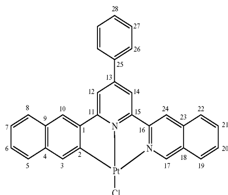
Complex 3
