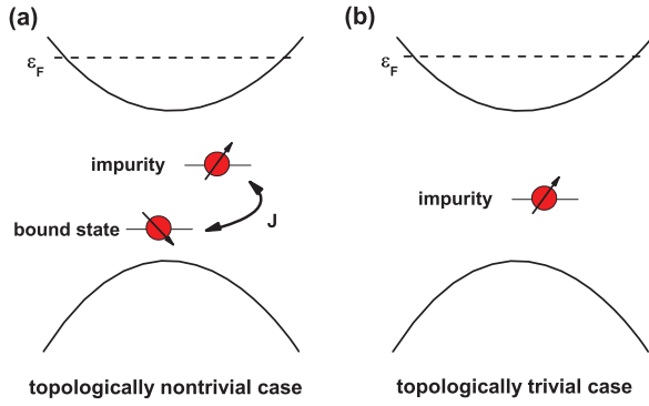
FIG. 7. (Color online) Illustration of the Kondo effect for (a) topological nontrivial case and (b) trivial case.
