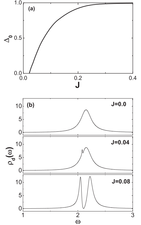
FIG. 8. (a) The order parameter \Delta_0 as a function of J . Parameters: \epsilon_d = 1.0 , \mu = 2.0 , and mB = 1.0 . (b) The density of states of the impurity for J = 0.0, 0.04, \text{ and } 0.08 .
