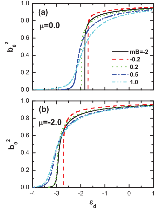
FIG. 6. (Color online) The dependence of the order parameter b_0^2 on the impurity energy level \epsilon_d for (a) the chemical potential in the gap \mu = 0.0 and (b) in the valence band \mu = -2.0 . Here mB = -2.0 and -0.2 represent the topological nontrivial case and mB = 0.2, 0.5 , and 1.0 correspond the topological trivial case.
