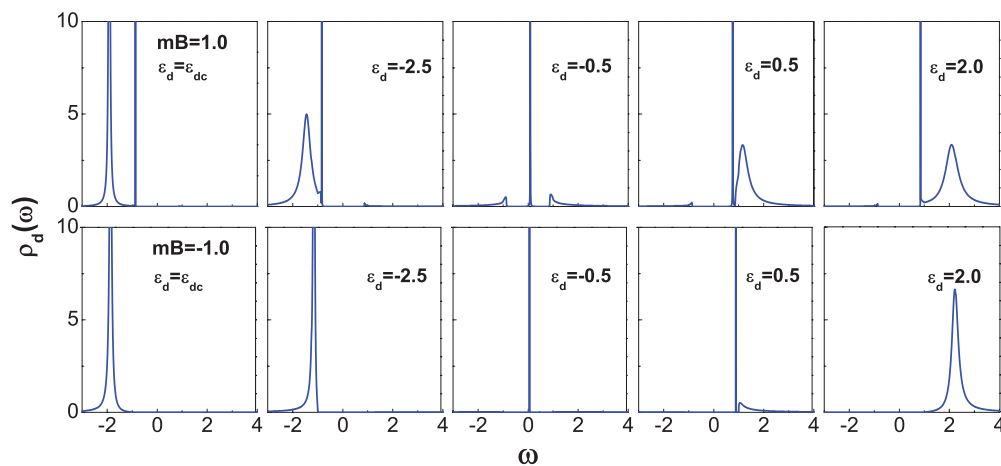
FIG. 4. (Color online) The density of states of the impurity electron is shown for different impurity levels \epsilon_d = \epsilon_{dc} ( \epsilon_{dc} is the critical point at which \tilde{\epsilon}_d = \mu ), -2.5, -0.5, 0.5 , and 2.0 (from left to right) in (a) topological nontrivial case mB = 1.0 and (b) topological trivial case mB = -1.0 , where the chemical potential \mu = -2.0 lies in the valence band.
