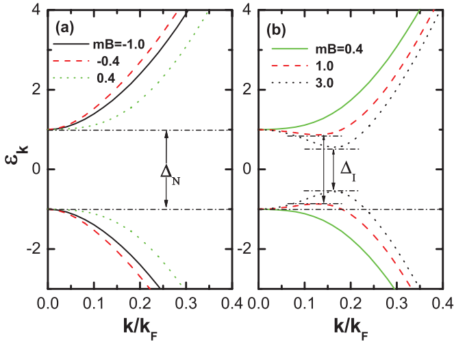
FIG. 1. (Color online) The energy spectrum \epsilon_k for different mB values: (a) mB = -1.0, -0.4, 0.4 ; (b) mB = 0.4, 1.0, 3.0 . Here mv_F^2 is taken as the energy unit. For mB < 1/2 , the energy gap is located at k = 0 and equals \Delta_N \equiv 2|m|v_F^2 . For mB > 1/2 , the energy gap is located at a finite k and equals \Delta_I \equiv \frac{\sqrt{4mB-1}}{|B|} v_F^2 .
