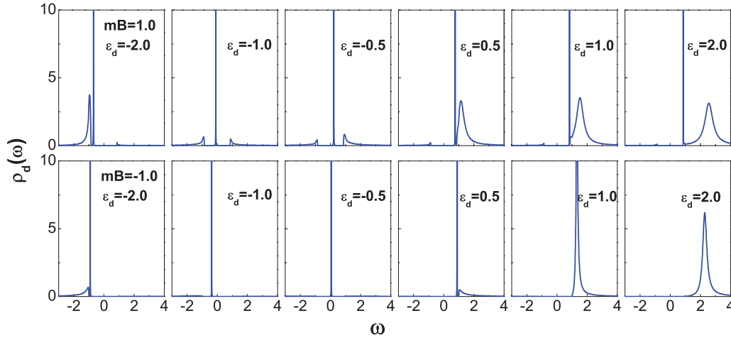
FIG. 3. (Color online) The density of states of the impurity electron is shown for different impurity levels \epsilon_d = -2.0, -1.0, -0.5, 0.5, 1.0 , and 2.0 (from left to right) in (a) topological nontrivial case mB = 1.0 and (b) topological trivial case mB = -1.0 , where the chemical potential \mu = 0.0 lies in the gap.
