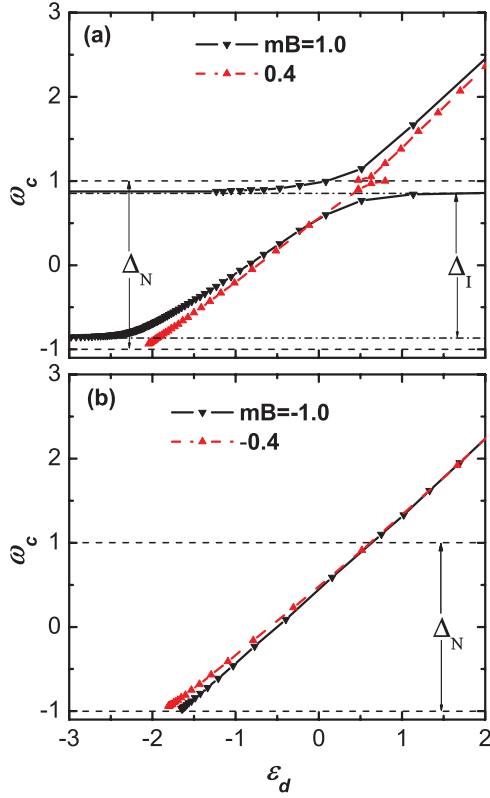
FIG. 5. (Color online) The positions of the bound states and low-energy Kondo resonance peak as functions of impurity level \epsilon_d in (a) the topological nontrivial case mB = 1.0, 0.4 and (b) the topological trivial case mB = -1.0, -0.4 . The chemical potential is taken as \mu = 0.0 .
