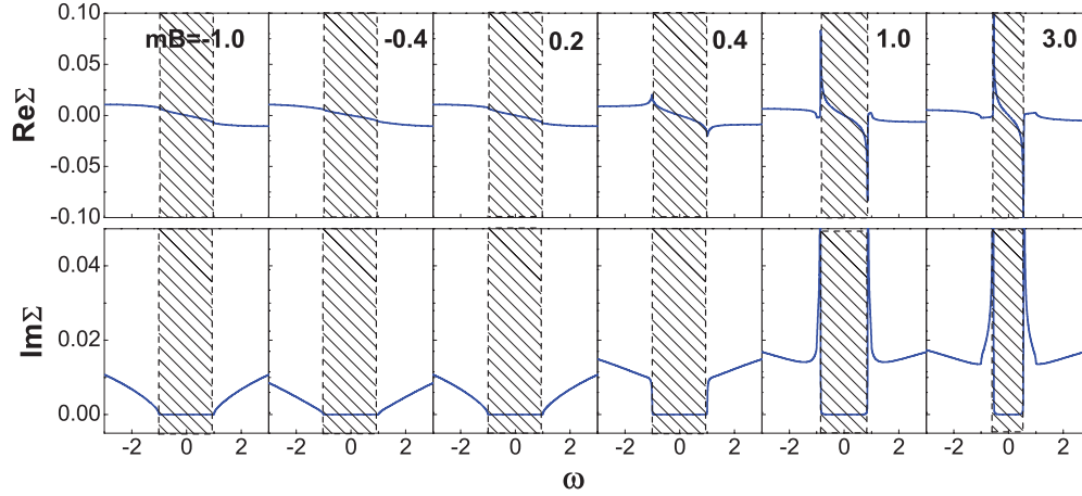
FIG. 2. (Color online) The real and imaginary parts of the self-energy \Sigma_0(\omega) for different mB values. The shaded part represents the region of energy gap.
