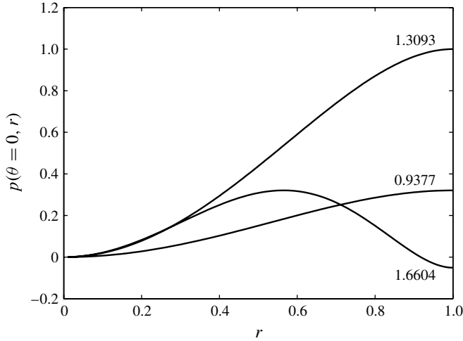
FIGURE 5. Pressure along the rotation axis, p(\theta = 0, r) , plotted according to the expression (3.1), for the three fundamental modes \hat{\omega}_{12} = 1.309 , \hat{\omega}_{13} = 0.9377 and \hat{\omega}_{23} = 1.6604 .
