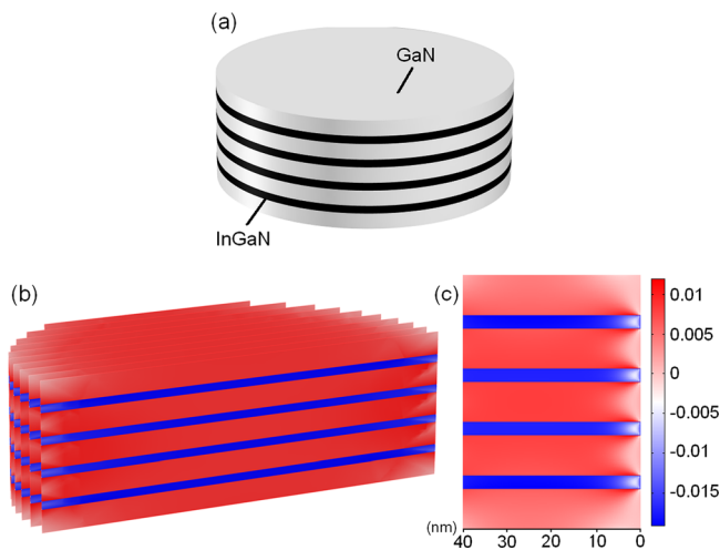
FIG. 6. (a) The disk model containing four pairs of InGaN/GaN QWs as used in the 3-D finite element strain simulations. (b) Simulated results showing the strain profile along the planes of the QWs. (c) Enlarged view showing strain distributions near the edge of the disk. The scale bar on the right represents the value of the in-plane strain.
