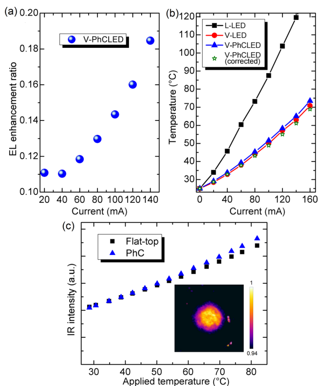
FIG. 4. (a) EL enhancement ratios of the V-PhCLED over the V-LED as calculated from the EL data of Fig. 2. (b) The variations of surface temperatures vs currents as measured by LWIR camera. (c) IR intensities as functions of applied temperatures. The inset shows the LWIR image illustrating intensity contrast between the PhC (circular central region) and the flat-top GaN surface (outside the central region). The scale bar on the right represents the normalized LWIR intensity.
