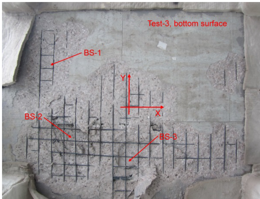
(b) Soffit spalling
