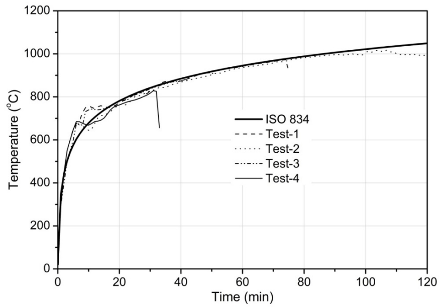
Figure 6: Furnace fire curves and standard fire curve
