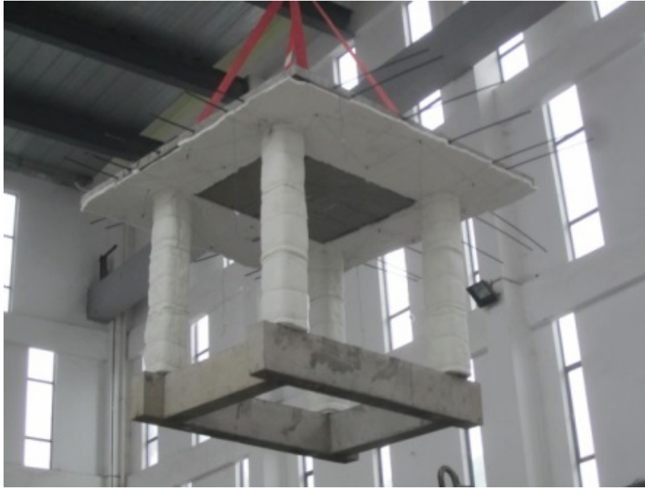
Figure 1: Overview of one test specimen
