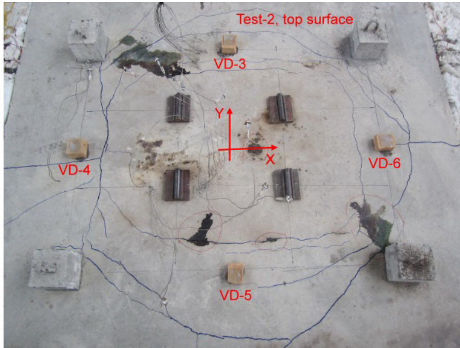
(a) Cracks at top surface after fire
