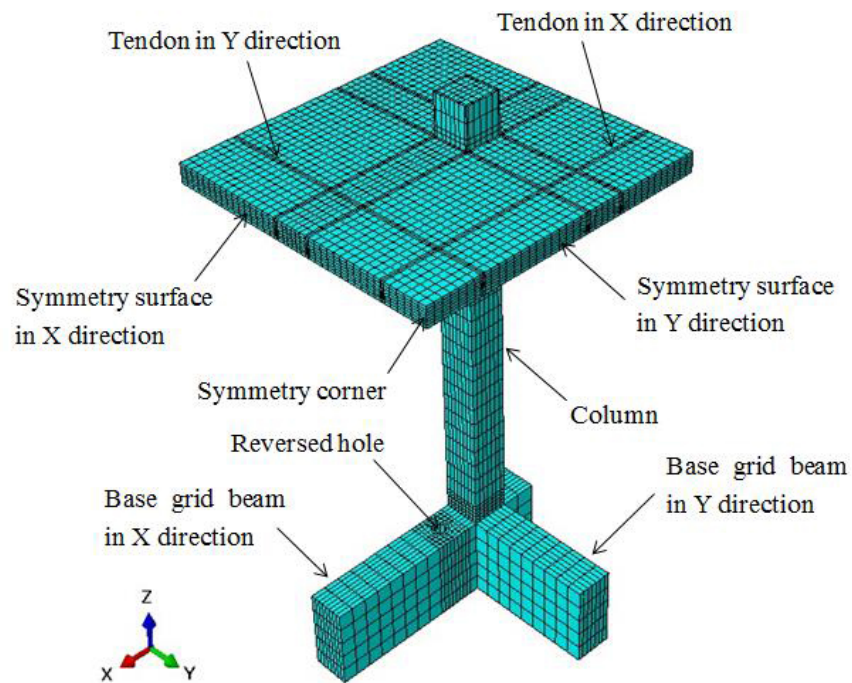
Figure 2: Numerical model of a quarter of specimen
