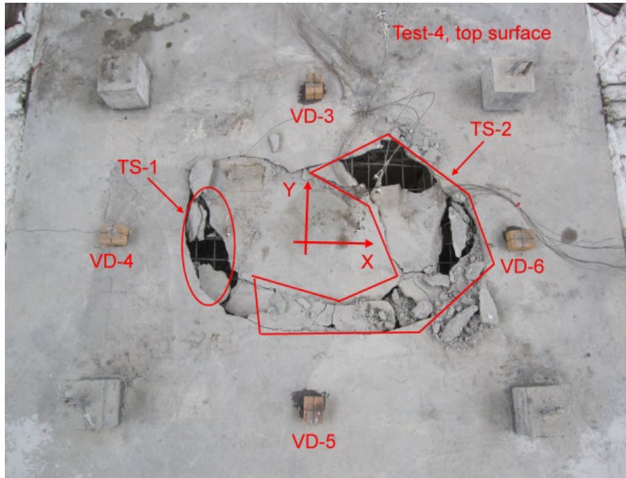
(a) Top surface spalling
