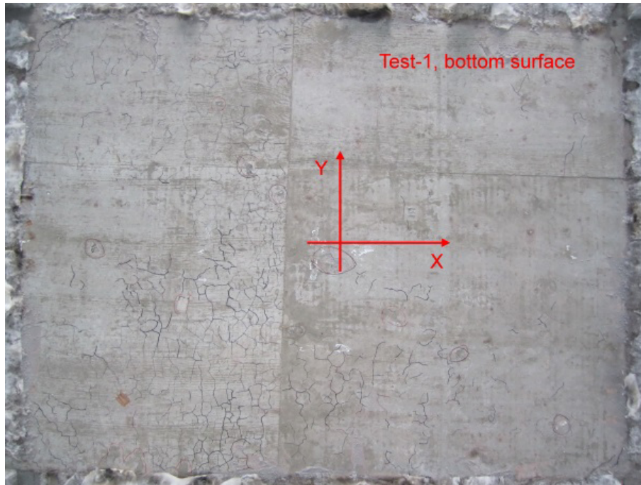
(c) Cracks at soffit after fire
