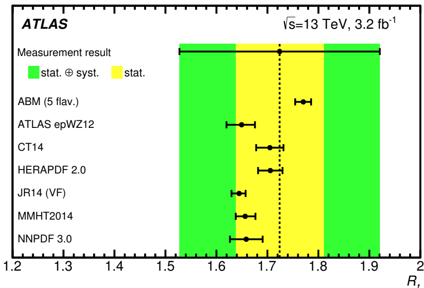
Figure 6. Comparison between observed and predicted values of R_t = \frac{\sigma_t}{\sigma_{\text{top}}} . Predictions are calculated at NLO precision [7, 8] in the five-flavour scheme and given for different NLO PDF sets. The uncertainty includes the uncertainty in the renormalisation and factorisation scales, as well as the combined internal PDF and \alpha_s uncertainty. The dotted black line indicates the measured value. The combined statistical and systematic uncertainty of the measurement is shown in green, while the statistical uncertainty is represented by the yellow error band. Predictions for all presented PDF sets are within the statistical uncertainty of the measurement.
