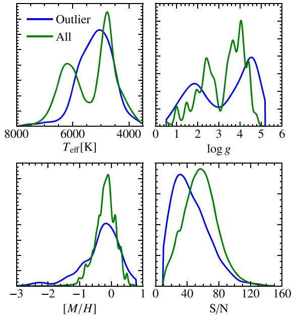
Figure 10. Distributions of the quoted parameters of the \sim 1000 stars that are outliers in the sense that they have |\Delta| > 4 (blue lines), and of all stars in the study, for reference (green lines). The plots are pdfs (so the area is normalized to 1 in all cases) produced using a kernel density estimate. The distributions shown are in T_{\text{eff, IRFM}} (top left), \log g_{\text{DR5}} (top right), [M/H] (bottom left), and S/N (bottom right). The outliers cover a wide range of these parameter spaces, and do not come from any clearly distinct population.
