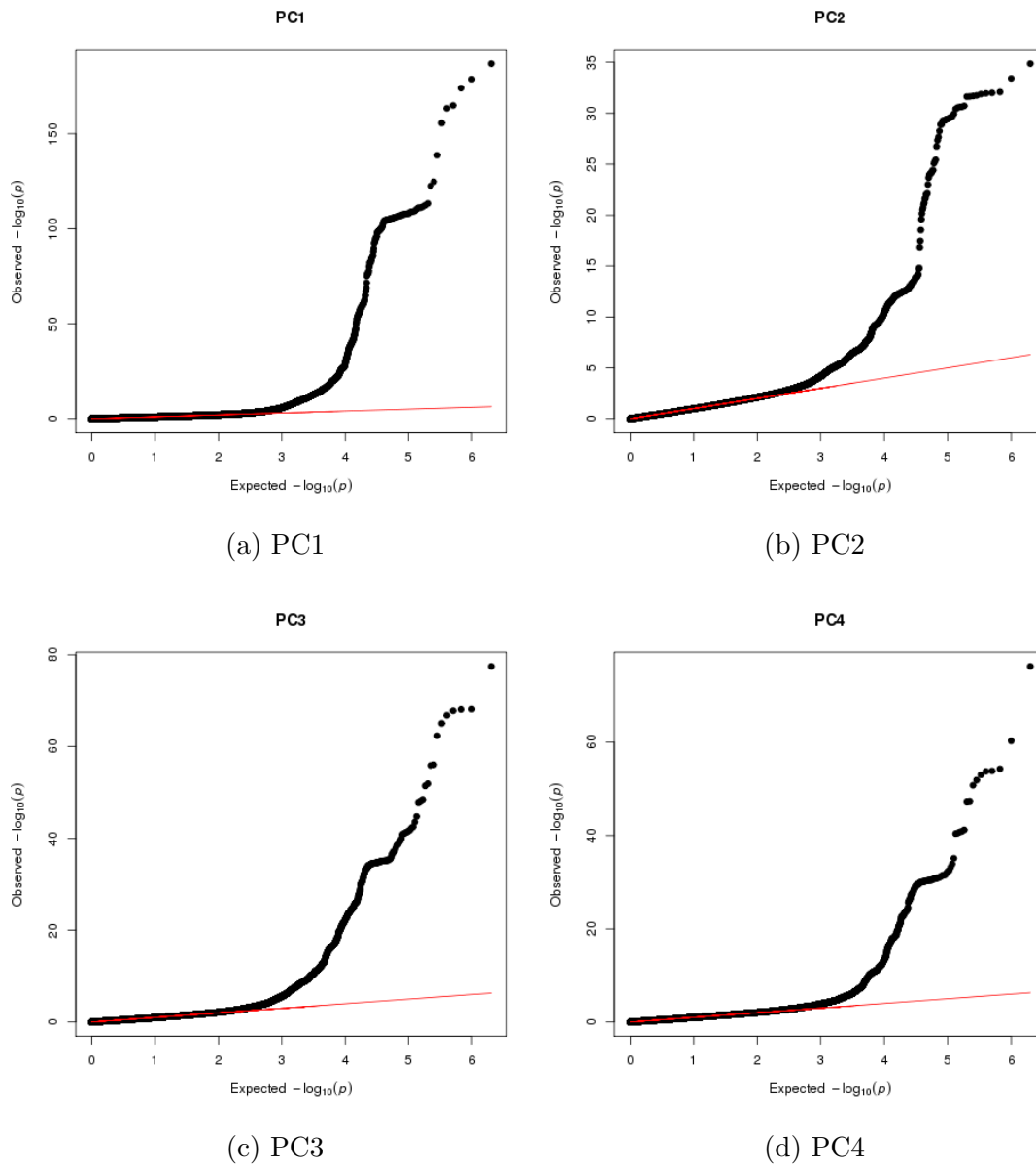
Figure S5. QQ plots for the p-values of PC1, PC2, PC3 and PC4.
