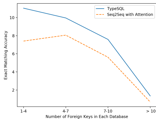
Figure 4: Exact matching accuracy as a function of the number of foreign keys.
