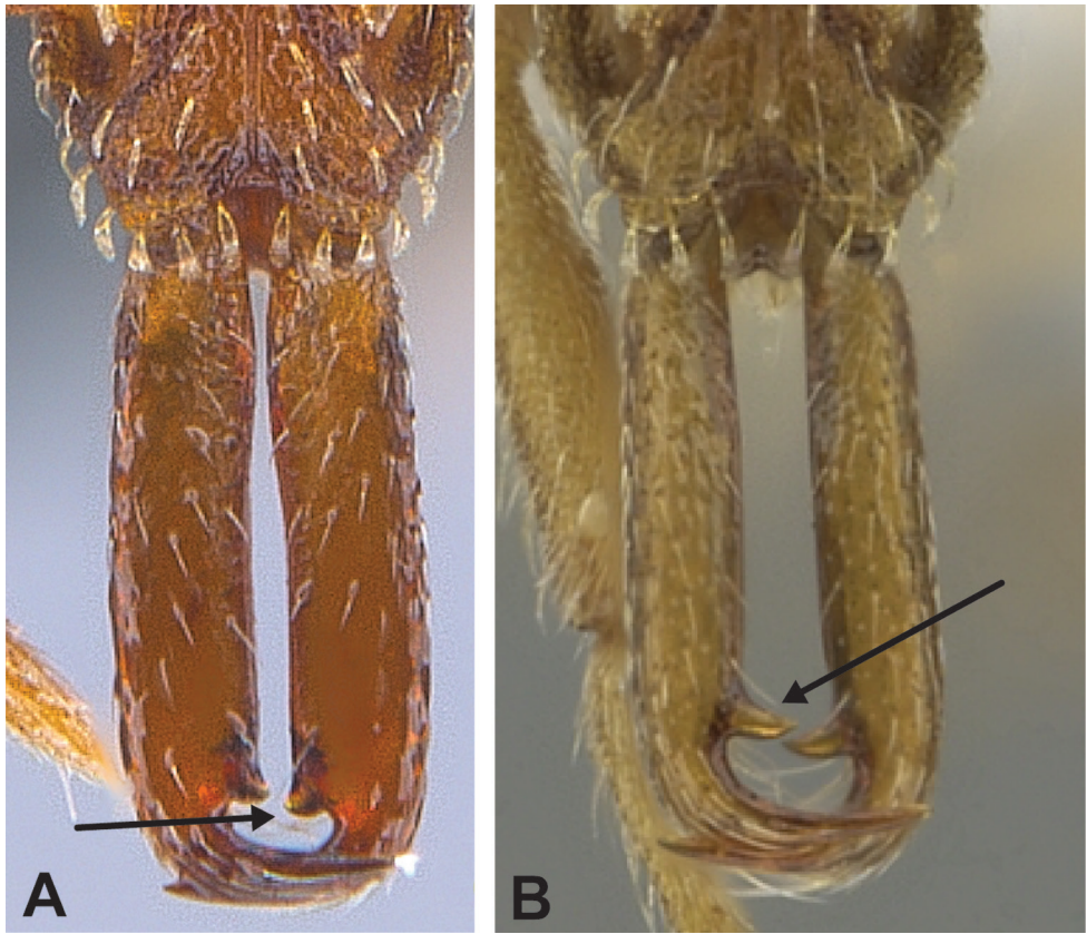
Figure 57. Examples of small preapical tooth in S. feae ( A MAC_S15_LLSP_sp.8, photographed by IBBL) and of larger preapical tooth in S. stenorbina ( B CASENT0900840, photographed by Ryan Perry).
