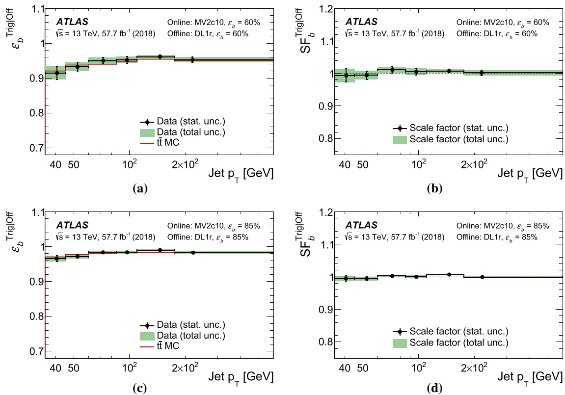
Fig. 14 The conditional b -tagging efficiency, \varepsilon_b^{\text{Trig/Off}} , (a, c) and corresponding scale factor, SF_b^{\text{Trig/Off}} , (b, d) for the online MV2c10 algorithm for the 60% efficiency working point (a, b) and the 85% efficiency working point (c, d) as measured in 2018 data. Offline jets are required
