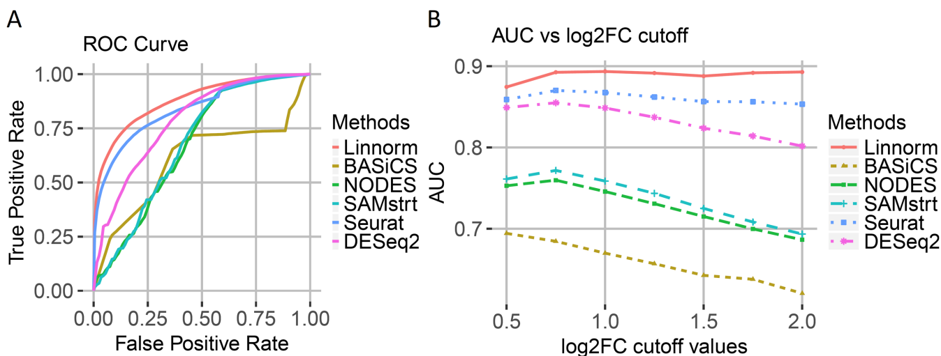
Figure 7. DEG analysis performance with the SEQC dataset. (A) Receiver operating characteristic (ROC) curve of SEQC DEG analysis using a sample set size of 10. True DEG are defined as genes with absolute \log_2 -fold change ( \log_2\text{FC} ) higher than 1 in the gold standard Taqman dataset. (B) Area under the ROC curve across Taqman \log_2\text{FC} s from 0.5 to 2.
