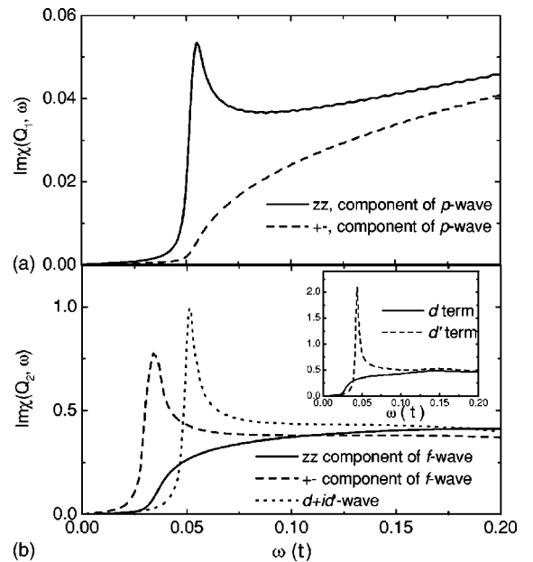
FIG. 2. Frequency dependence of \text{Im} \chi in the SC state ( T=0.0001t ): (a) for the p_x+ip_y wave at n=1.35 and \mathbf{Q}_1 ; (b) for the f and d+id' waves at n=0.4 and \mathbf{Q}_2 . The inset of (b) shows the results for the pure d and d' waves, respectively.
