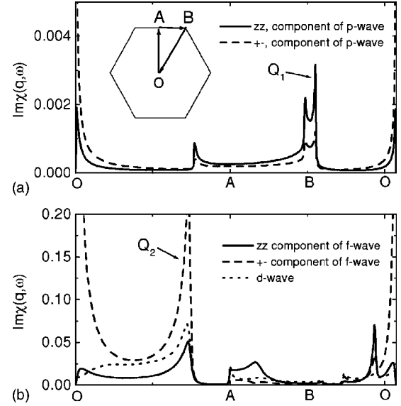
FIG. 1. Momentum dependence of \text{Im} \chi with \omega=0.02t for (a) p_x+ip_y wave at n=1.35 , and (b) f and d+id' waves at n=0.4 . The momentum is scanned along the path shown in the inset of (a).
