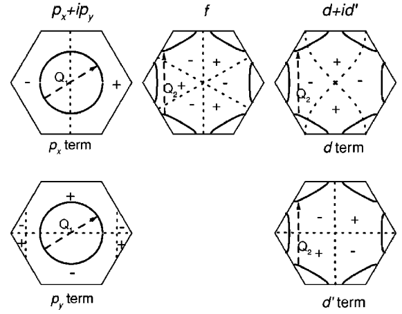
FIG. 4. Fermi surface (thick lines) and phase ( \pm ) of the gap functions for three possible pairing symmetries. The dotted lines denote the node positions that separate the regions with different phases, and the dashed lines with arrows represent the transition wave vectors \mathbf{Q}_1 and \mathbf{Q}_2 as indicated in Fig. 1.
