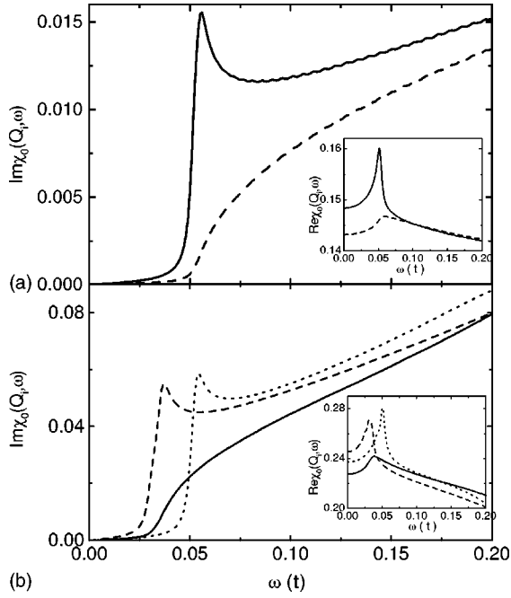
FIG. 3. Frequency dependence of the bare spin susceptibility \chi_0 in the SC state ( T=0.0001t ): (a) the p_x+ip_y wave at n=1.35 and \mathbf{Q}_1 , where the solid line indicates \text{Im} \chi_{zz}^0 and the dashed line \text{Im} \chi_{+-}^0 ; (b) the f and d+id' waves at n=0.4 and \mathbf{Q}_2 , where the solid line indicates \text{Im} \chi_{zz}^0 of the f wave, the dashed line \text{Im} \chi_{+-}^0 of the f wave, and the dotted line the d+id' wave.
