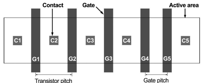
Fig. 3 Typical layout block of neighboring MOSFETs in a standard cell.
