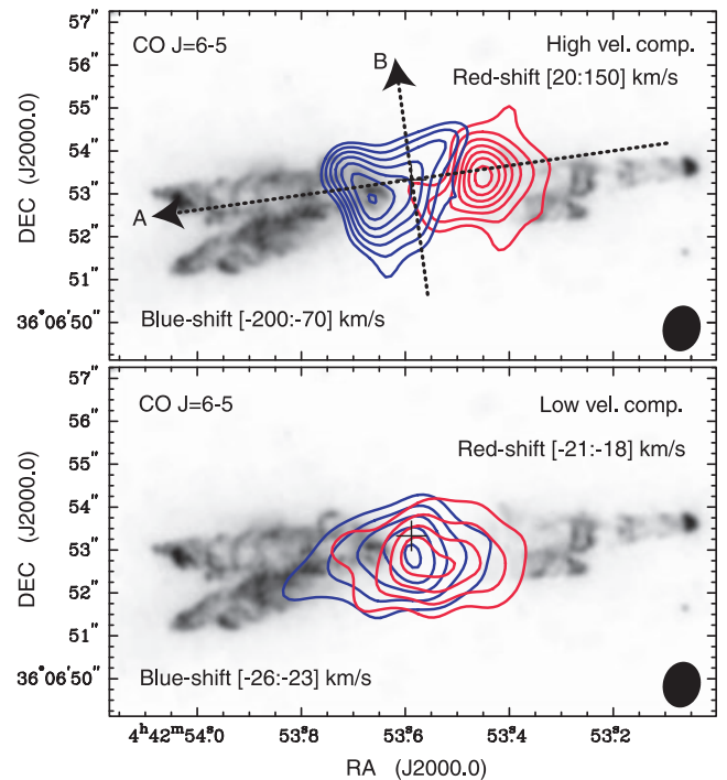
FIG. 4.—Velocity-integrated intensity maps of the CO J = 6-5 line superimposed on the HST WFPC2 \text{H}\alpha + continuum image (Trammell & Goodrich 2002). The red and blue contours represent the redshifted and blueshifted parts of the high- and low-velocity components. The velocity ranges of the integration are given in the panels. The lowest contour corresponds to the 3\sigma level, and the levels are spaced every 4\sigma ; the 1\sigma levels for the top and bottom panels are 1.2 \times 10^{-1} and 6.9 \times 10^{-1} \text{ Jy beam}^{-1} , respectively. The synthesized beam size is given in the lower right corner. The dotted arrows A and B indicate the directions along which the p - v cuts shown in Fig. 8 were taken.
