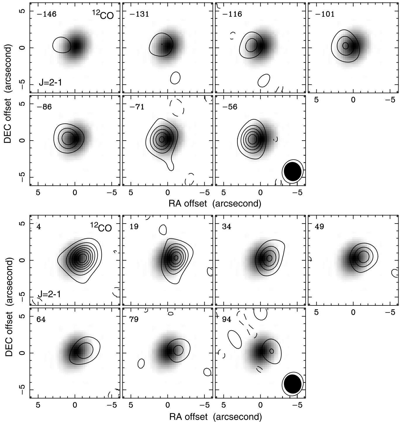
FIG. 7.—Velocity channel maps of the high-velocity component of the CO J = 2-1 line. The velocity channels are averaged over 1 \text{ km s}^{-1} intervals. The contours start from the 3 \sigma level, and the levels are spaced every 10 \sigma . The dashed contour corresponds to -3 \sigma . The 1 \sigma level, background gray scale, and synthesized beam are the same as in Fig. 6.
