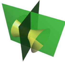
Fig. .4. The case of QSIC having two real conics intersecting in two real points.
