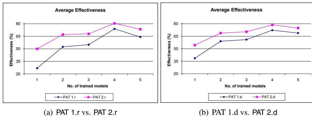
Figure 8: Effectiveness of PAT 2.r over PAT 1.r, and PAT 2.d over PAT 1.d
