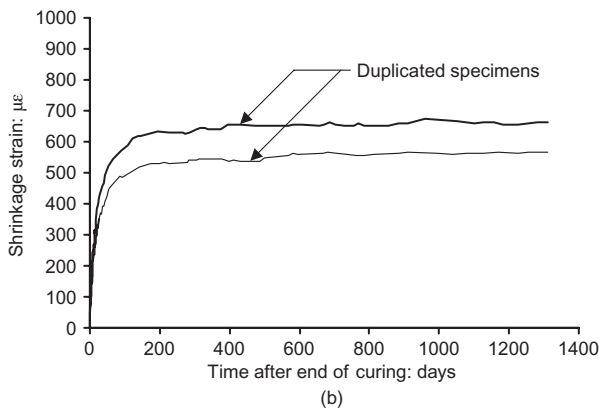
Figure 3. Shrinkage–time curves of some concrete mixes at RH = 75%: (a) mix 1; (b) mix 2
