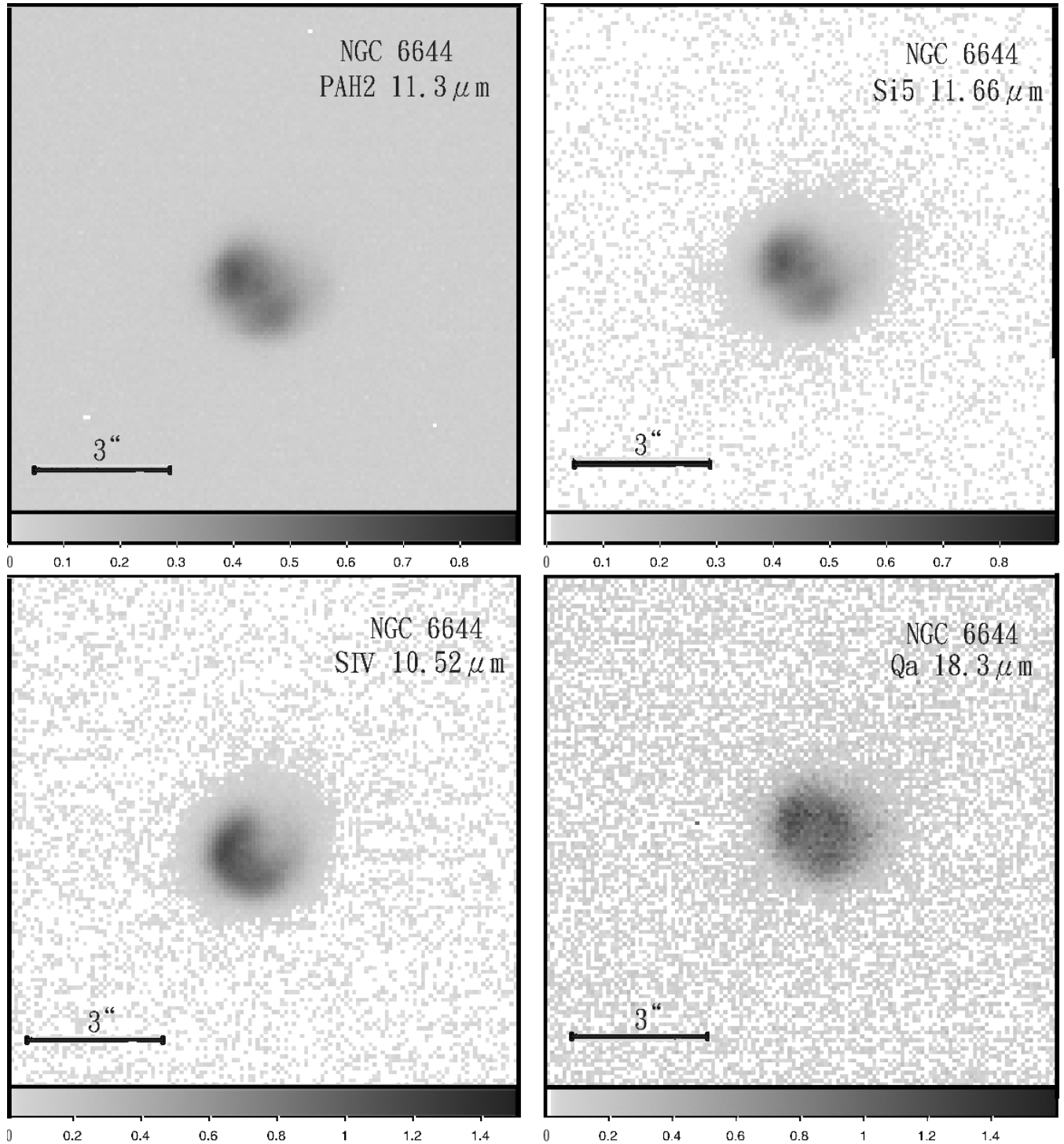
Fig. 8.— Flux-calibrated Gemini T-ReCS images of NGC 6644. The four panels give respectively the PAH-2 11.3 \mu\text{m} image (upper left), the Si5 11.66 \mu\text{m} image (upper right), [S IV] 10.52 \mu\text{m} narrow-band image (lower left), and Q_a 18.3 \mu\text{m} medium-band image (lower right). North is up and East is to the left. The intensity display is on a linear scale and the grey scale bar is given at the bottom in units of counts per pixel.
