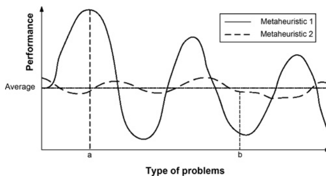
Fig. 2. Comparison of performance for different problem types.
