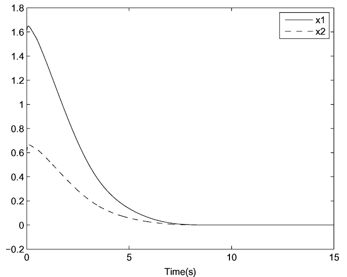
Fig. 2. State response of the uncertain system.
