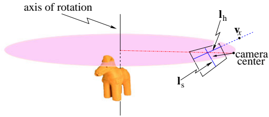
Figure 1: Under circular motion and fixed intrinsic parameters of the camera, the image of the rotation axis I_s , the horizon I_h and the vanishing point v_x will be fixed throughout the sequence. The fundamental matrix relating any pair of views in the sequence can be parameterized explicitly in terms of these fixed features.
