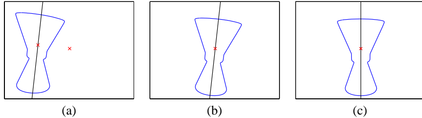
Figure 2: (a) The harmonic homology associated with the silhouette of the surface of revolution is estimated, which yields the image of the revolution axis. The image is then normalized by \mathbf{K}^{-1} , and the orthogonal projection \mathbf{x}_0^p of the point \mathbf{x}_0 = [0 \ 0 \ 1]^T on the image of the revolution axis is located. (b) The image is transformed by the homography \mathbf{R}_b so that the point \mathbf{x}_0 lies on the image of the revolution axis and the silhouette becomes bilaterally symmetric about the image of the revolution axis. (c) Finally, the image is rotated about the point \mathbf{x}_0 until the image of the revolution axis aligns with the y -axis.
