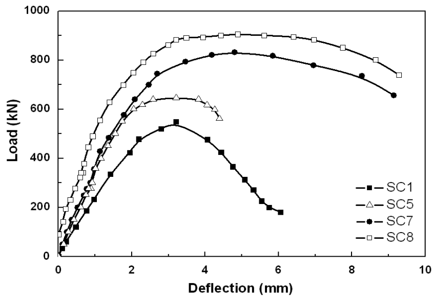
Figure 16 Load-deflection curves
