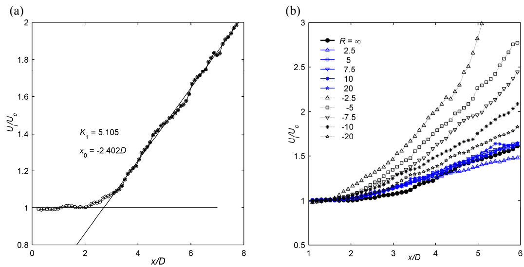
Fig. 3. Axial development of jet centerline velocity. (a) Simple jet data and fitted x^{-1} decay of Eq. (1): solid symbols showing data used in fitting. (b) Jets in co-flow and counter-flow (with negative R ), and simple jet ( R = \infty ).
