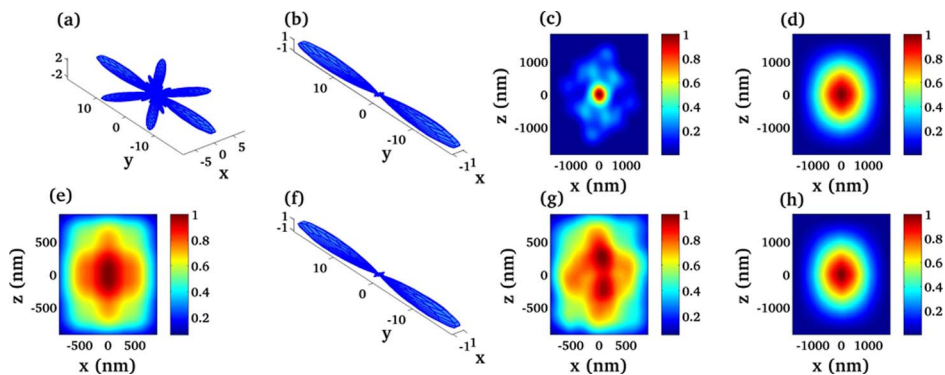
Fig. 3. (Color online) (a), (f), and (b) Radiation patterns of the reference NA and the optimized ones with and without random fabrication errors, respectively; (c), (h), and (d) spatial correlation functions of the E_z components for the reference NA and the optimized ones with and without random fabrication errors, respectively; (g), (e) near-field intensities of the optimized NAs with and without random fabrication errors, respectively.
