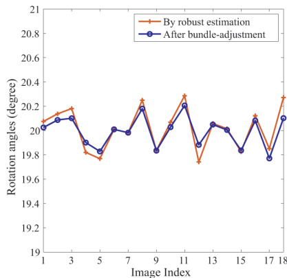
Fig. 13. Vase sequence: angles estimated using the robust method and those obtained after bundle adjustment. The RMS errors of the estimated rotation angles before and after the bundle adjustment are 0.134^\circ and 0.112^\circ , respectively.
