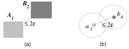
Fig. 5. Qualified combinations for the join. (a) Nonleaf combination. (b) Leaf combination.
