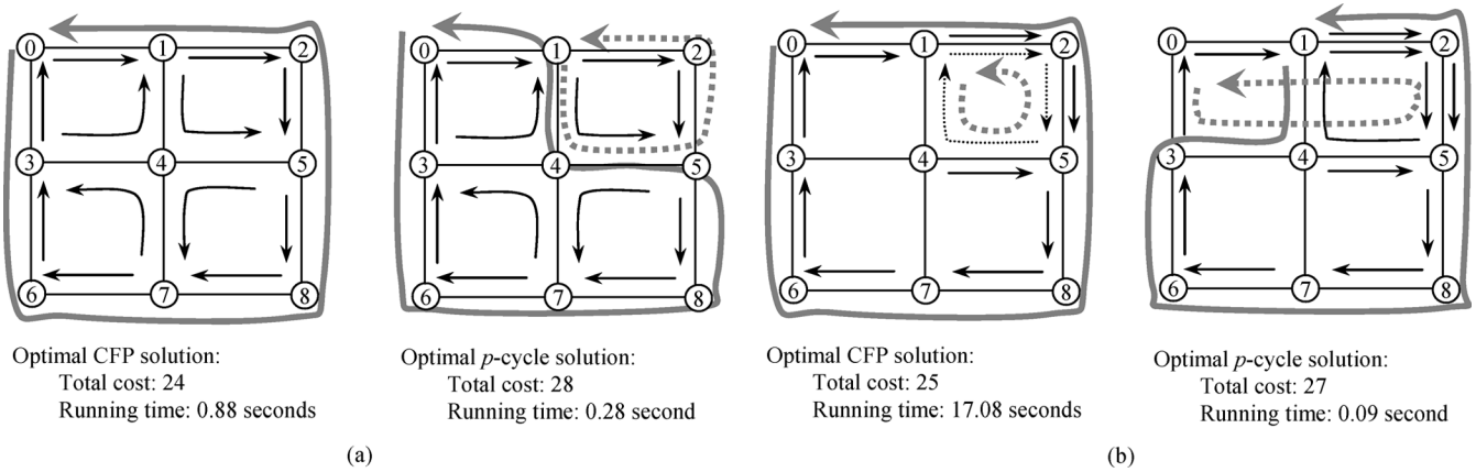
Fig. 7. CFP versus p -cycle protection in a 3 \times 3 Manhattan topology. (a) L = \{L_{sd}\} = \{L_{01} = 1, L_{12} = 1, L_{25} = 1, L_{58} = 1, L_{87} = 1, L_{76} = 1, L_{63} = 1, L_{30} = 1, L_{31} = 1, L_{15} = 1, L_{57} = 1, L_{73} = 1\} . (b) L = \{L_{sd}\} = \{L_{01} = 1, L_{12} = 2, L_{25} = 2, L_{58} = 1, L_{87} = 1, L_{76} = 1, L_{63} = 1, L_{30} = 1, L_{51} = 1, L_{45} = 1\} .
