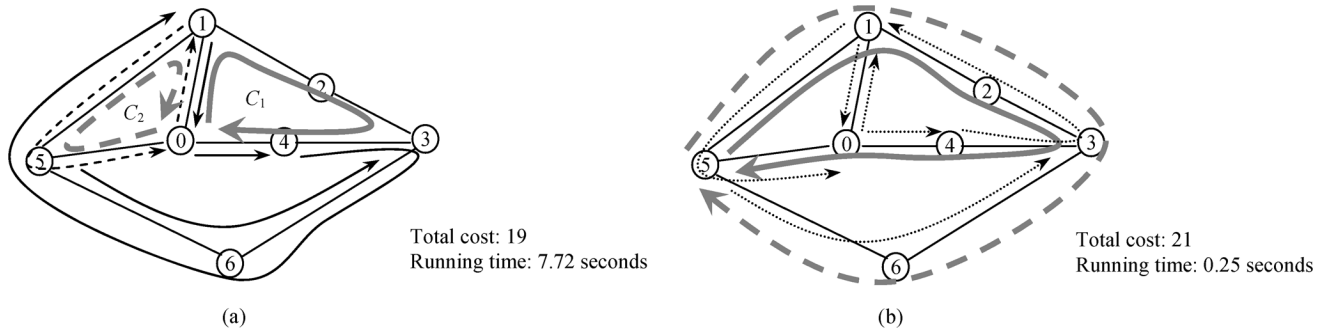
Fig. 6. A simple network with L = \{L_{sd}\} = \{L_{01} = 1, L_{04} = 1, L_{10} = 2, L_{41} = 1, L_{53} = 1\} . (a) Optimal CFP solution. (b) Optimal p -cycle solution.
