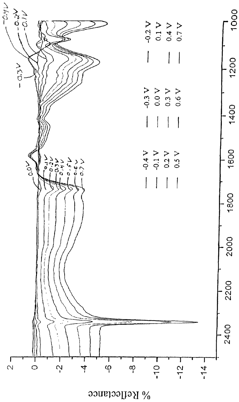
Wavenumber / cm -1
