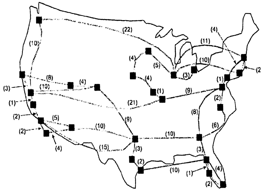
Fig. 10. The AT&T North America OC-48 fiber network obtained in March 2001 from the URL http://www.ipservices.att.com/backbone/bbone-map.cfm .
