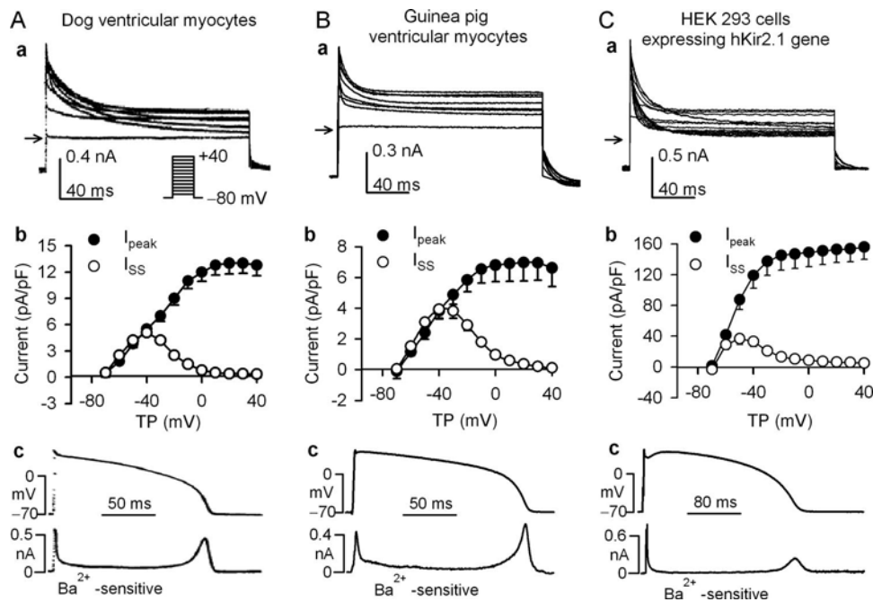
Fig. (1). Ba 2+ -sensitive transient outward component of cardiac I K1 channels activated by depolarization. A-a. Ba 2+ -sensitive current was recorded in a dog ventricular myocyte, and obtained by digitally subtracting the currents before and after application of 200 μM Ba 2+ . Membrane currents were elicited with the voltage protocol shown in the inset. The arrow indicates the 0 current level. A-b. I-V relationships of the peak current ( I peak , measured from current peak to 'quasi'-steady-state level) showed intermediate inward rectification, while that of steady-state current ( I SS , measured from holding current to the 'quasi'-steady-state level) exhibited strong inward rectification (middle panel). A-c. Action potential (recorded from a dog ventricular myocyte) waveform clamp revealed two components of Ba 2+ sensitive current. B-a. Ba 2+ -sensitive current recorded in a guinea pig ventricular myocytes with same protocol as shown in the inset of A-a. B-b. I-V relationships of I peak and I SS showed similar properties to those in dog ventricular myocytes. A-c. Action potential (recorded from a guinea pig ventricular myocyte) waveform clamp also revealed two components of Ba 2+ sensitive current. C-a. Ba 2+ -sensitive current recorded in a HEK 293 cell stably expressing human Kir2.1 gene with same protocol as shown in the inset of A-a. C-b. I-V relationships of I peak and I SS in HEK Kir2.1 cell line showed similar properties to those in dog and guinea pig ventricular myocytes. C-c. Action potential (recorded from a human ventricular myocyte) waveform clamp also revealed two components of Ba 2+ sensitive current in HEK cells stably expressing Kir2.1 gene. Modified from Li GR, et al , 1998; 2000; and Zhang DY, et al , 2009 [42, 59, 60].
