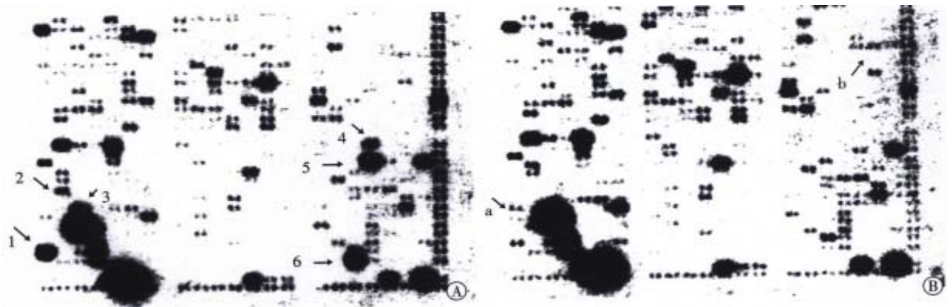
Figure 3 cDNA array: Differential gene expression in gastric mucosa of normal control rat (A) and sleep deprivation rat (B). Sleep deprivation may decrease the following genes expression (Arrow 1-6): 1: bile-salt-stimulated lipase; 2: pancreatic lipase related protein 2 precursor; 3: triacylglycerol lipase precursor; 4: elastase 2 precursor; 5: trypsinogen II; 6: chymotrypsinogen B precursor, and increase the following genes expression (Arrow a-c): a: low-density lipoprotein receptor precursor; b: glucose transporter type 1; c: transferrin receptor protein. The dot for over expressed inducible heat shock protein 70 gene is circled.
