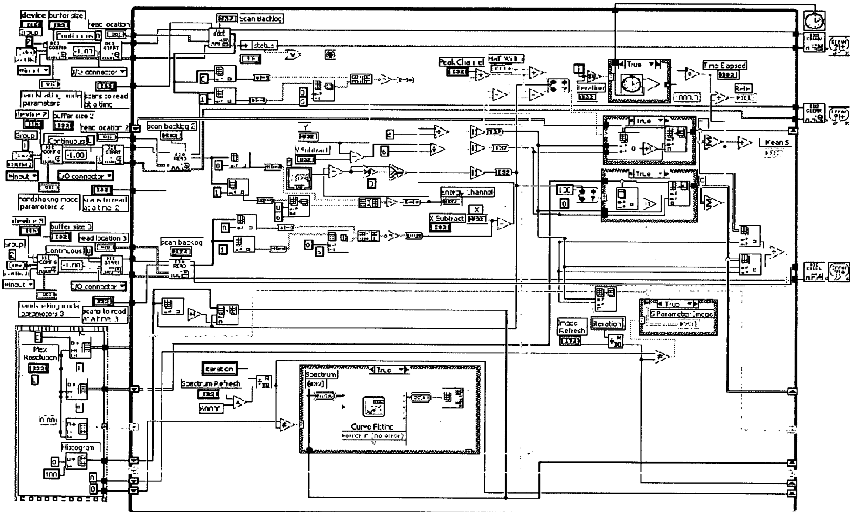
Figure 3 : VI diagram of the complete imager software.
