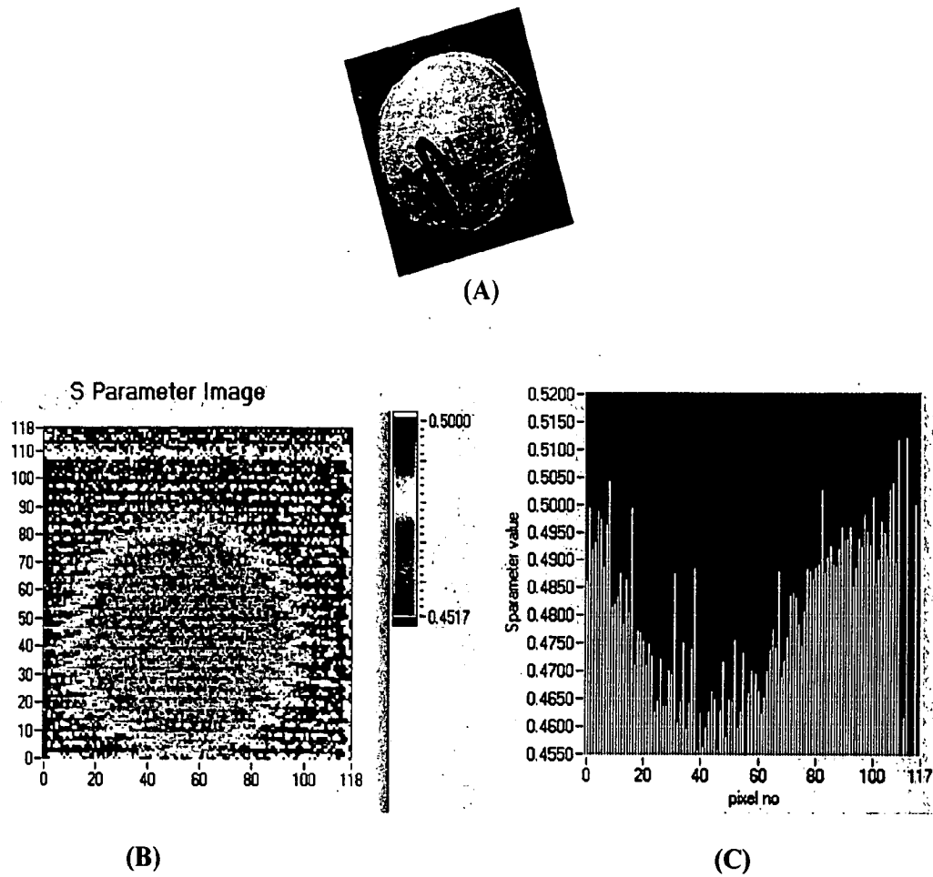
Fig 9 : Monocrystalline Ni sample produced by high pressure torsion by Paul Scherrer Institute , Switzerland. (A) Photo graph (B) S-parameter image (C) Bar-chart plotting of the S-parameter value versus the pixel number with the data values taken along row 55 from Fig 9B.
