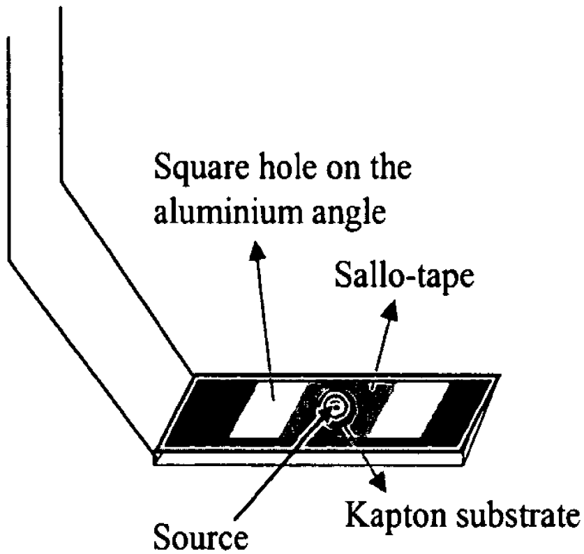
Fig 11 : Top view of the sample holder
