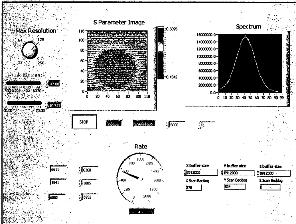
Fig 4 : Front Panel of the imager software.
