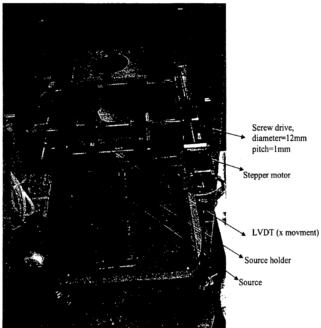
Fig-13 : Photograph of the scanning apparatus : side view.
