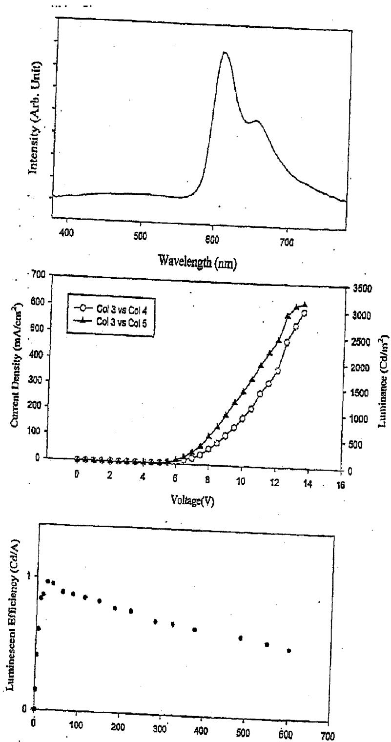
Figure 10. Electroluminescent spectrum, current-voltage (I-V) and luminance-voltage (B-V) curves and luminescent efficiency-current density curve of the device using complex 16 as emitter with a doping level of 4%.
