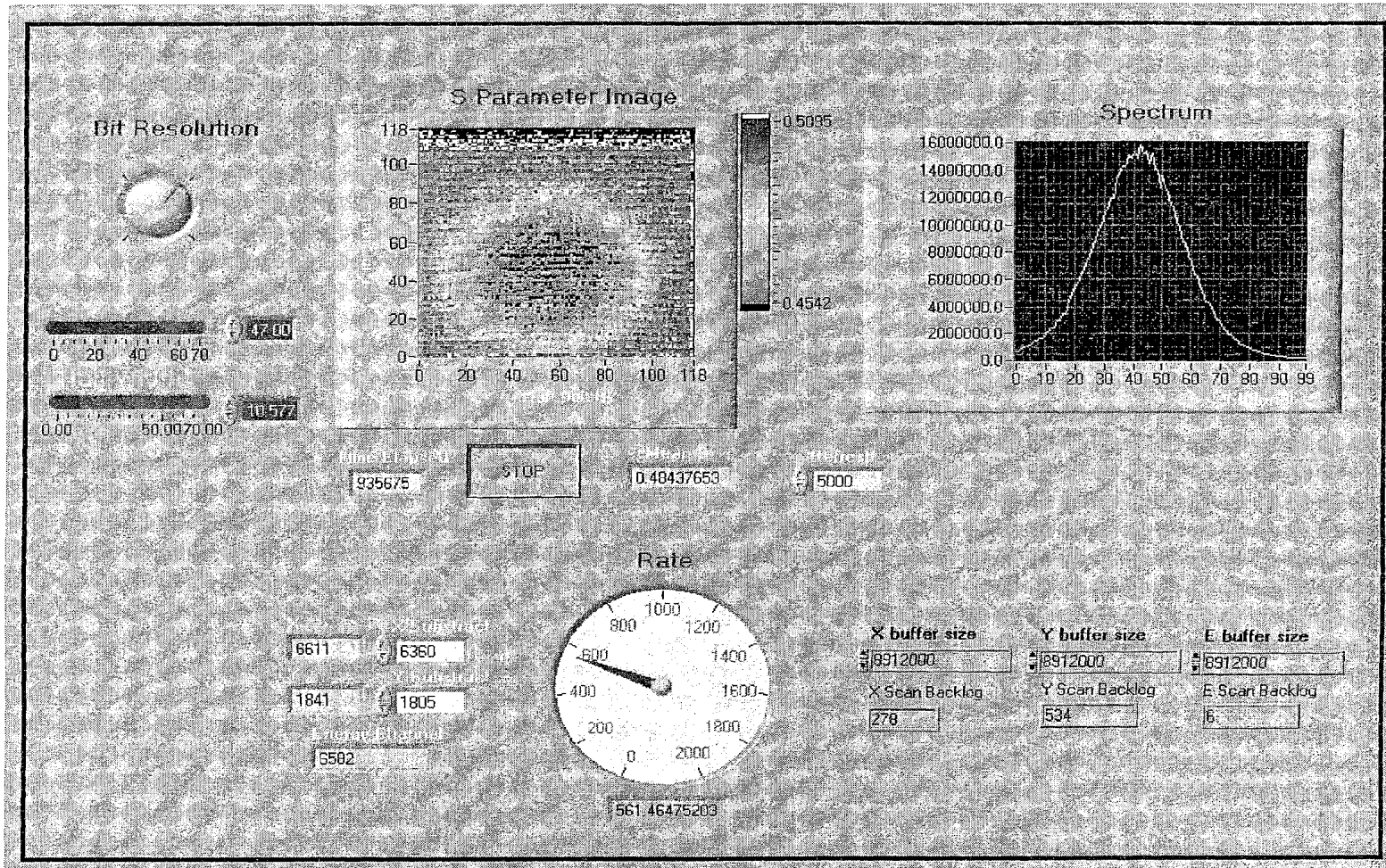
Fig. 4 : Front Panel of the imager software.
