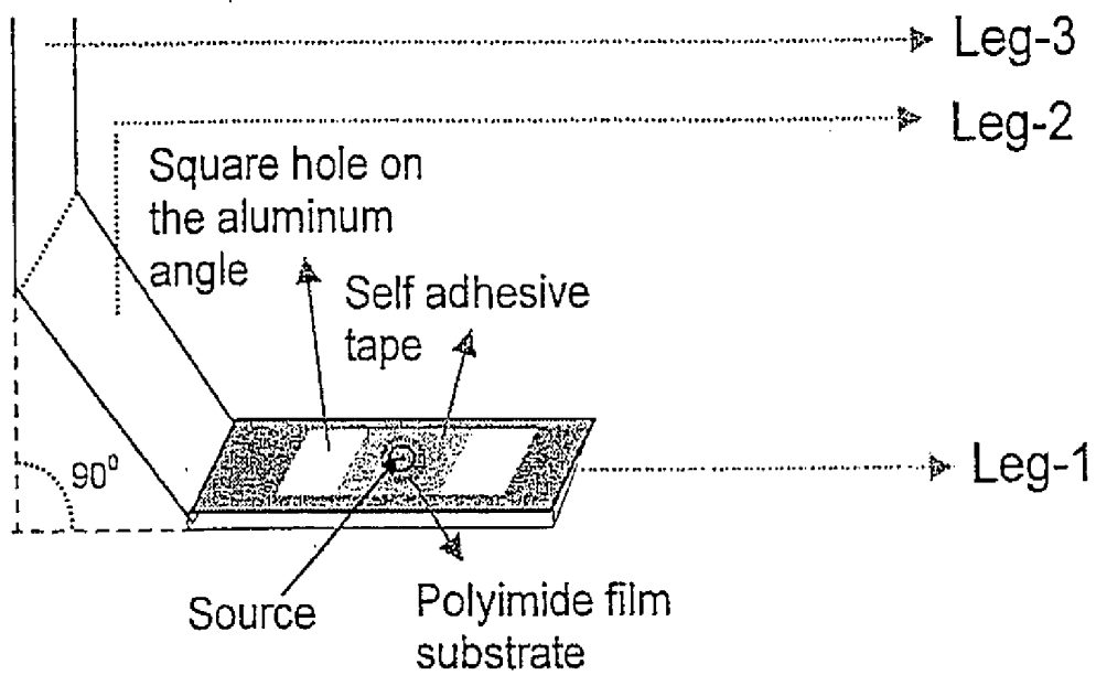
Fig 11 : Top view of the sample holder
