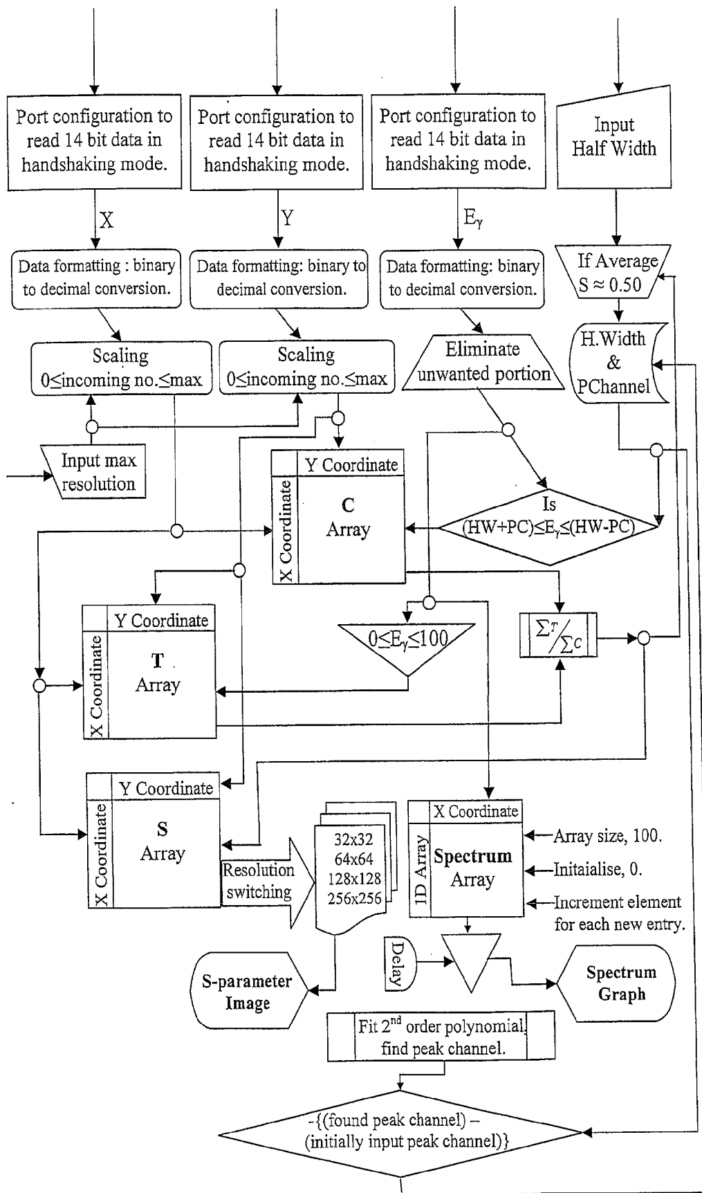
Fig. 20 : The System software : a flow chart representation.
