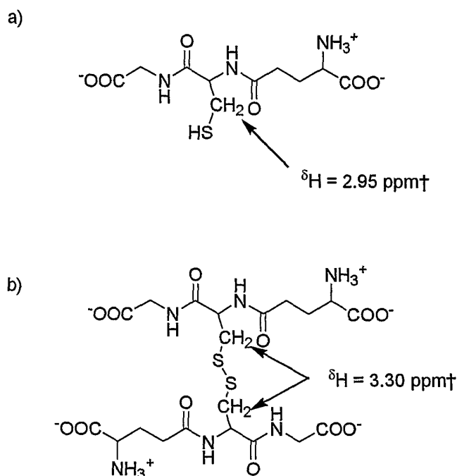
Scheme 5. Characteristic proton resonance absorptions for (a) GSH and (b) GSSG in D 2 O
