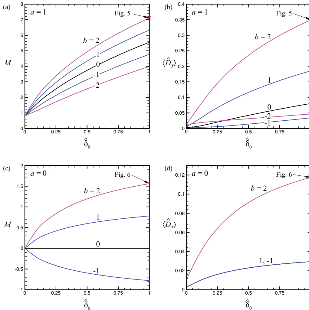
FIG. 4. For non-uniform slip ( \sigma = 1 ) and \hat{\kappa} = 10 , (a) and (c) the mobility M , and (b) and (d) the averaged dispersion coefficient ( \hat{D}_T ), as functions of the slip length \hat{\delta}_0 , where a = 1 in (a) and (b) and a = 0 in (c) and (d). See Figs. 5 and 6 for the cases marked with a symbol.
