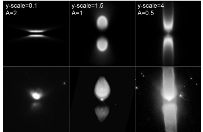
Figure 12. Top row: a simulation of evolutionary progression in morphology as the lobes get larger and the density of the dust halo drops. Evolution in age is from left to right. The model parameters are given in each of the three panels. A Gaussian convolution was applied to simulate the diffraction pattern of the telescope. Bottom row: observed images selected as examples of possible observational counterparts of the simulated images. From left to right: IRAS 13557–6442 (image created from NASA/ESA/STScI, Hubble Archives, Project GO9463, PI: Sahai); IRAS 19343+2926 (image created from NASA/ESA/STScI, Hubble Archives, Project GO6533, PI: Buharrabal); IRAS 10178–5958 (image created from NASA/ESA/STScI, Hubble Archives, Project GO6816, PI: Sahai).
