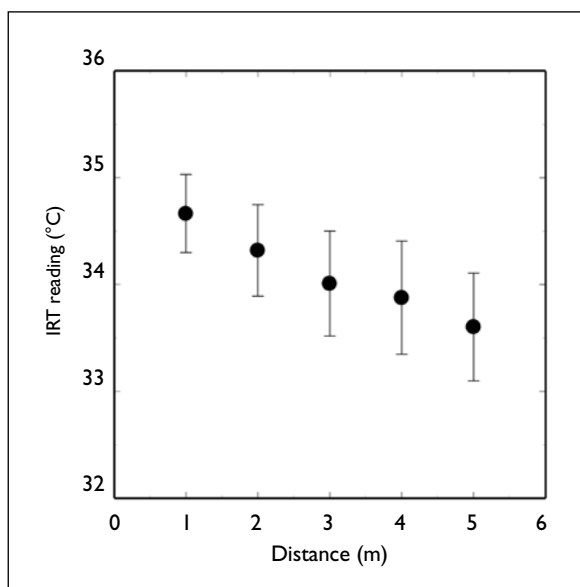
FIG 3. Relationship between infrared thermographic (IRT) temperature and distance of measurement Regression: IRT temperature ( ^{\circ}\text{C} ) = 34.85 - 0.26 distance (m)
