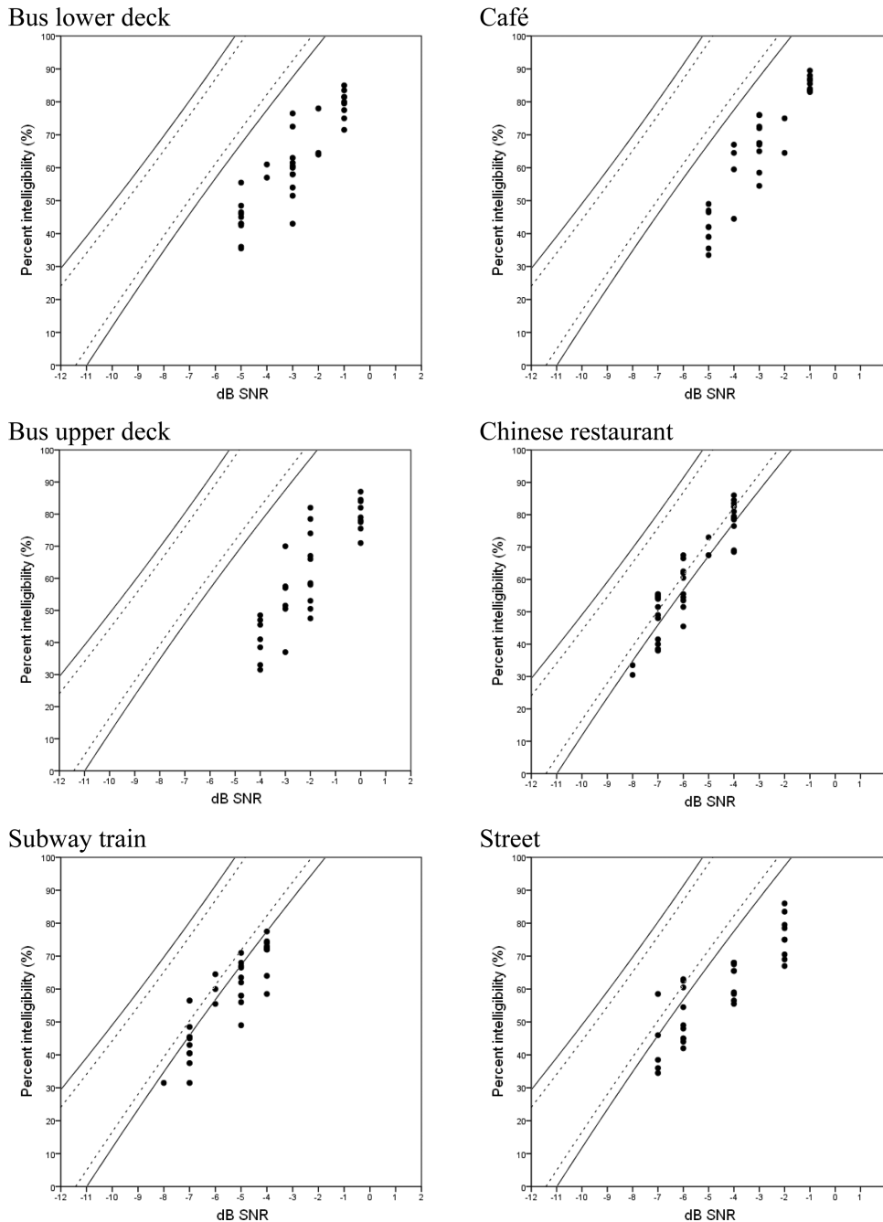
FIG. 4. Scatter plots of SNR-intelligibility score data points. The dashed lines and solid lines represent the 95% and 99% CI of the slope obtained from testing in steady-state speech-spectrum-shaped noise.
