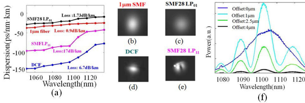
Fig. 2. (a) Measured GVD curves and the loss values of different fiber modes in the FMFs and the 1\mu\text{m} SMF. (b)-(e) Captured images of the fiber output mode patterns using the NIR camera. (f) Measured output spectra of the SMF28 when an alignment offset is varied at the fiber input. The fringes are attributed to the beating between the fundamental mode ( \text{LP}_{01} ) and higher-order mode ( \text{LP}_{11} ).
