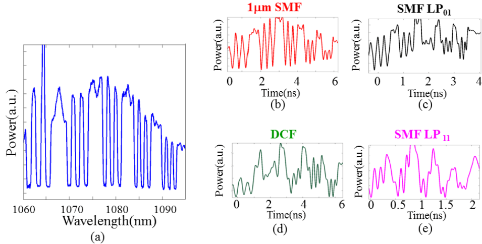
Fig. 3. Wavelength-to-time mapping based on different FMF modes as well as the 1\mu\text{m} SMF. (a) The input shaped spectrum to the fiber-under-test. The time-stretched signals of (b) 1\mu\text{m} SMF, (c) \text{LP}_{01} of SMF28, (d) \text{LP}_{01} of DCF and (e) \text{LP}_{11} of SMF28. The input misalignment offset is 4 mm in (d). Note that all the spectral information can in general be mapped into time well within few ns in all of the cases – demonstrating the ultrafast spectral acquisition speed enabled by the time-stretch process.
