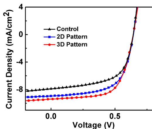
FIG. 2. Current density-voltage ( J - V ) characteristics of devices with or without nanopatterned back reflector measured under AM 1.5 illumination at 100 mW/cm 2 .
