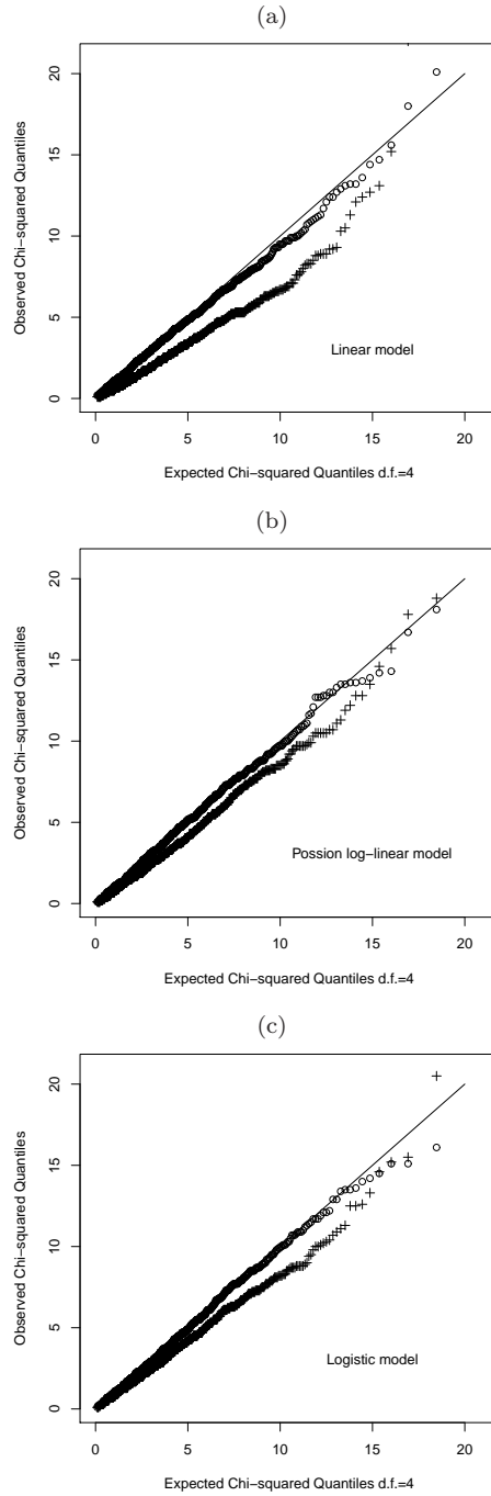
FIG 1. Quantile-quantile plots for the bootstrap \chi^2 test statistics with sample size n = 100 and K = 5 (“circle” representing the proposed \chi^2_{(K-1)} statistics based on the bootstrap sample MLE, and “+” representing the classical Pearson statistics based on the original data MLE): (a) the linear regression model; (b) the Poisson log-linear model; and (c) the logistic model.
