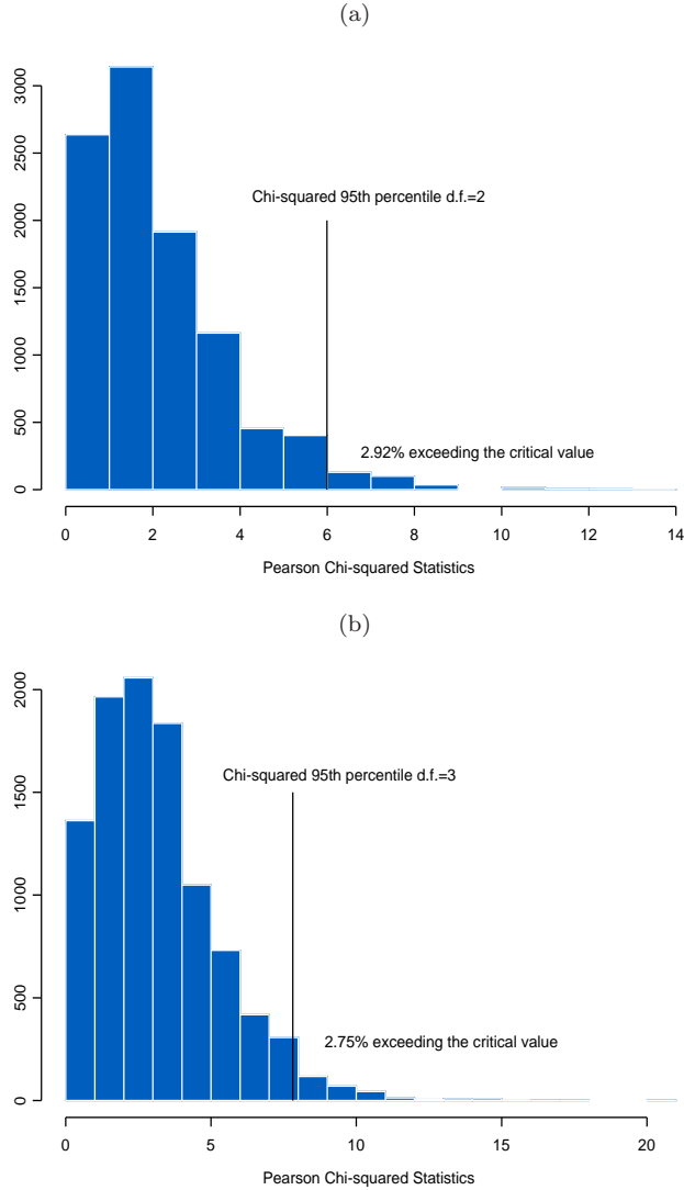
FIG 2. Histograms of the Pearson-type goodness-of-fit test statistics for the steam data with (a) K = 3 and (b) K = 4 .
