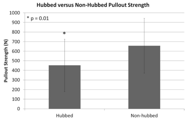
Hubbed vs. non-hubbed pedicle screw pullout strength (452±274N vs. 656±285N)
