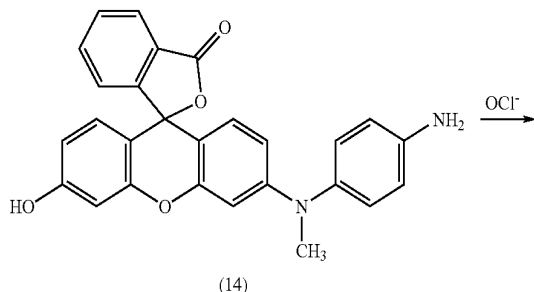
Scheme 7
